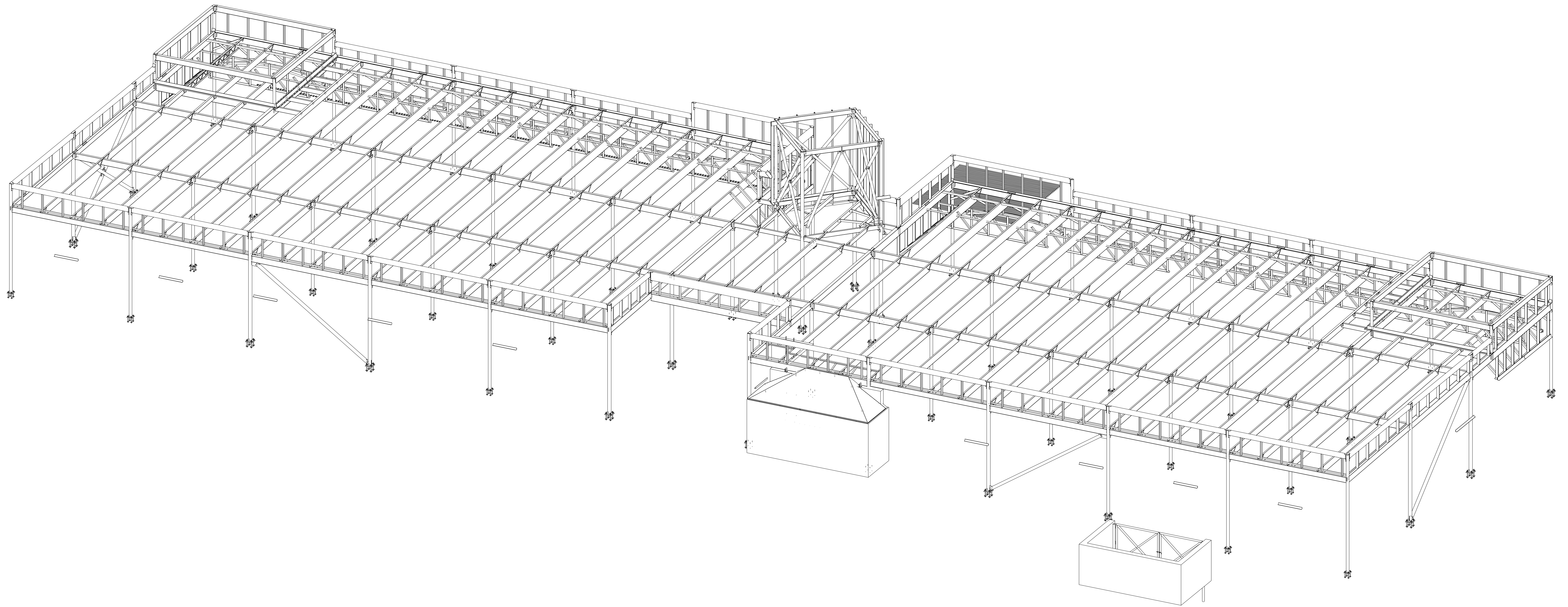
ISOMETRIC VIEW
